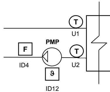
Water cooled detail
