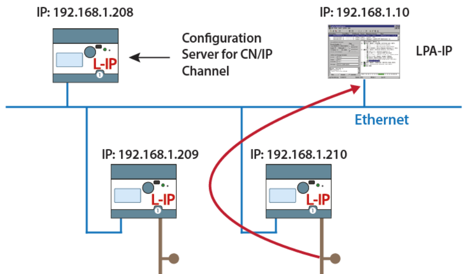
Figure 96: Remote LPA principle.
