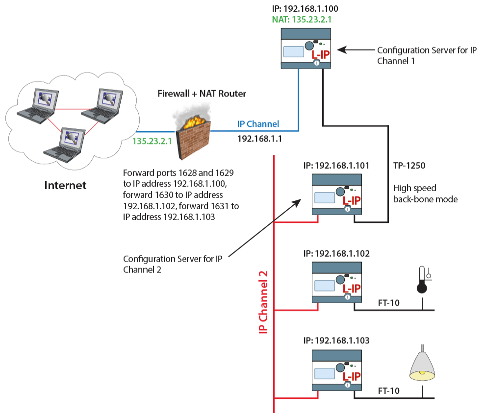
Figure 88: Application that uses multiple L-IP devices behind a NAT router firewall.
