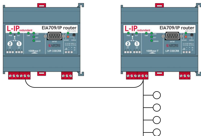
Figure 6: L-IP Redundant in Twin Router mode without Bus Loop Monitoring
