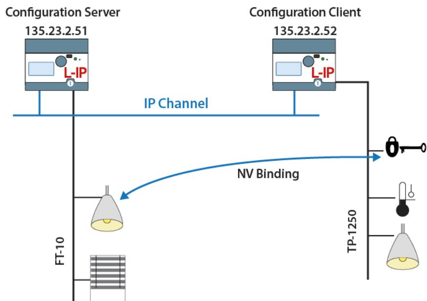
Figure 83: IP channel that consists of two IP devices. The left L-IP with IP address 135.23.2.51 acts as router and as a configuration server for this IP channel. It manages both IP devices 135.23.2.51 and 135.23.2.52.
