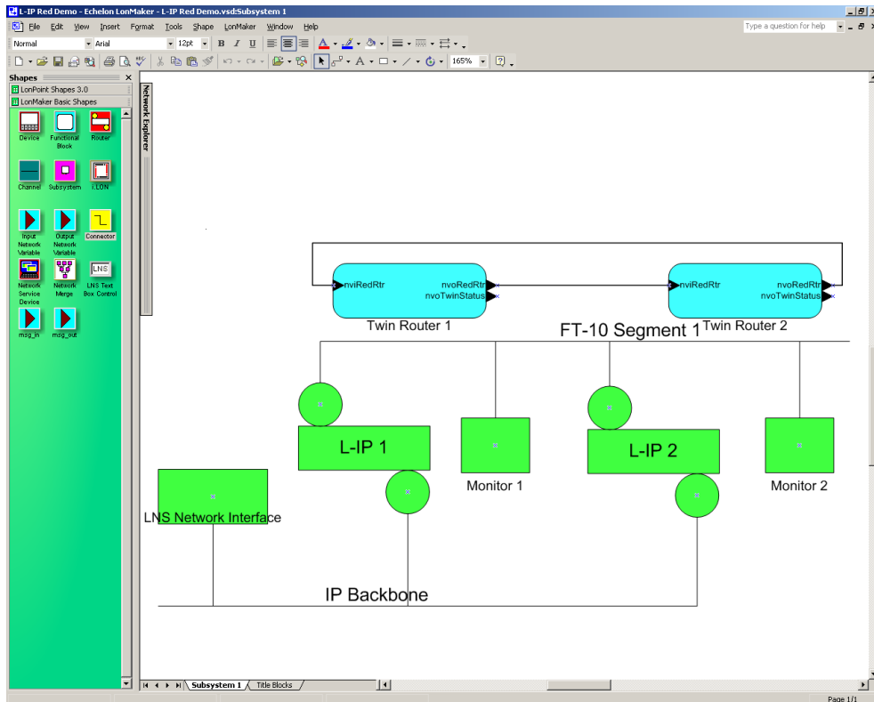
Figure 109: A pair of L-IP Redundant devices configured for twin router operation.
