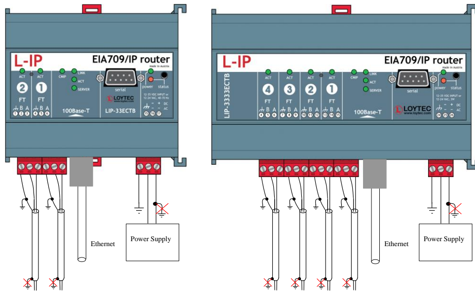
Figure 23: Connecting the Earth Ground to the L-IP series “B”.
