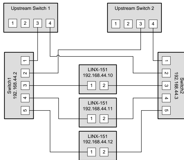
Figure 143: Fully redundant Ethernet topology
