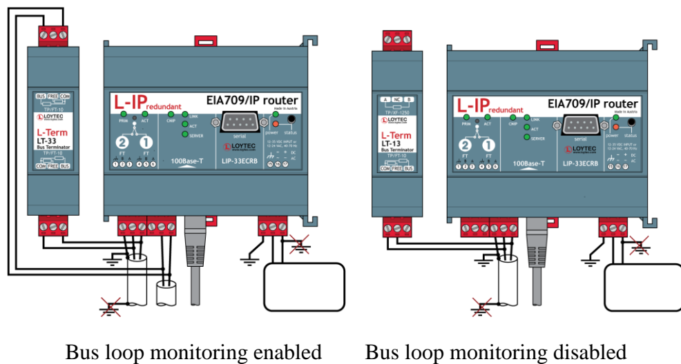
Figure 24: L-IP Redundant with and without Bus loop Monitoring
