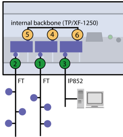
Figure 15: Internal assignment of NIDs on LIP-xxECTB.
