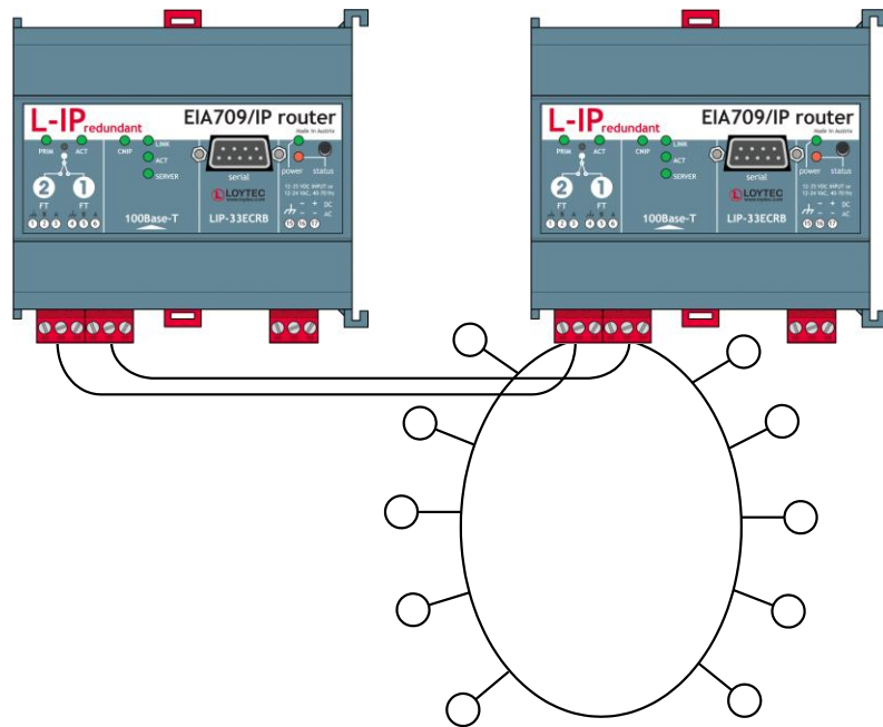
Figure 5: L-IP Redundant in Twin Router mode with Bus Loop Monitoring
