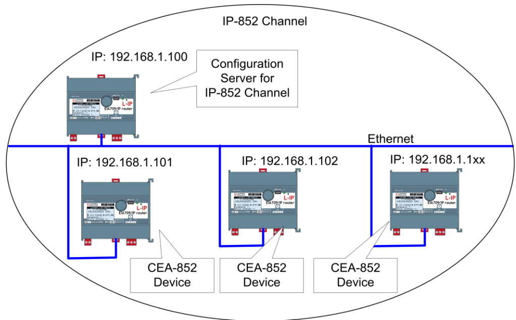
Figure 84: The configuration server manages the devices on an IP-852 channel.
