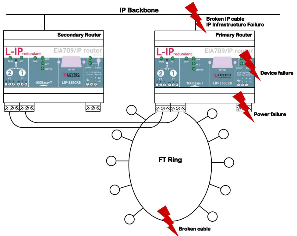
Figure 99: Router Redundancy with two paired L-IP Redundant routers
