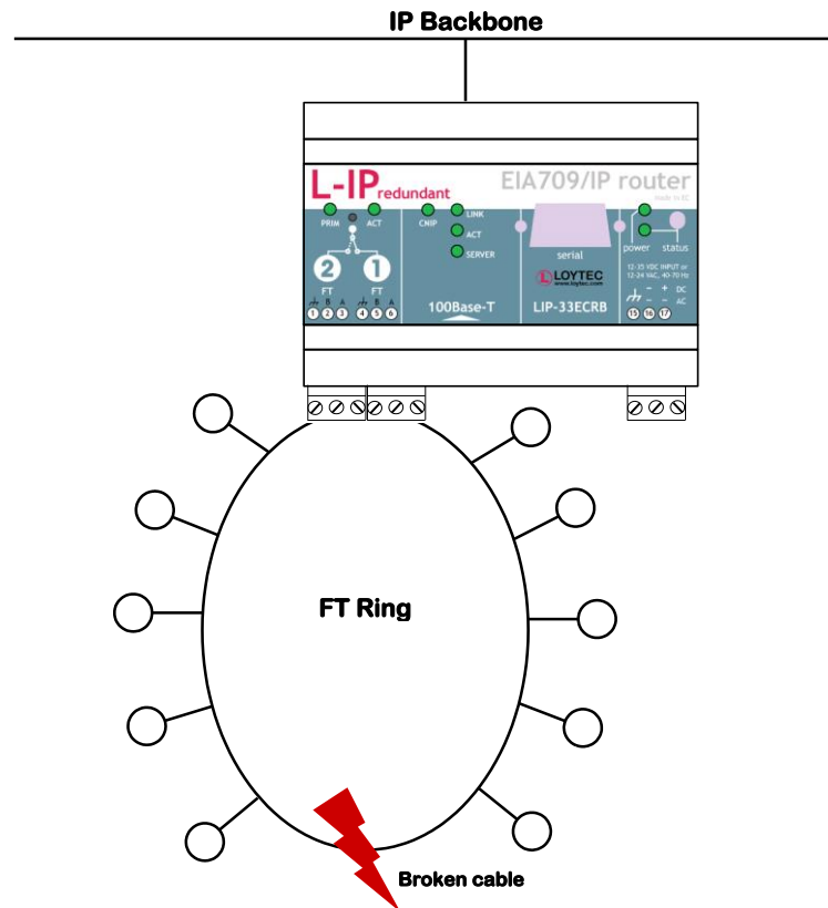
Figure 98: L-IP Redundant with Bus Loop Monitoring.
