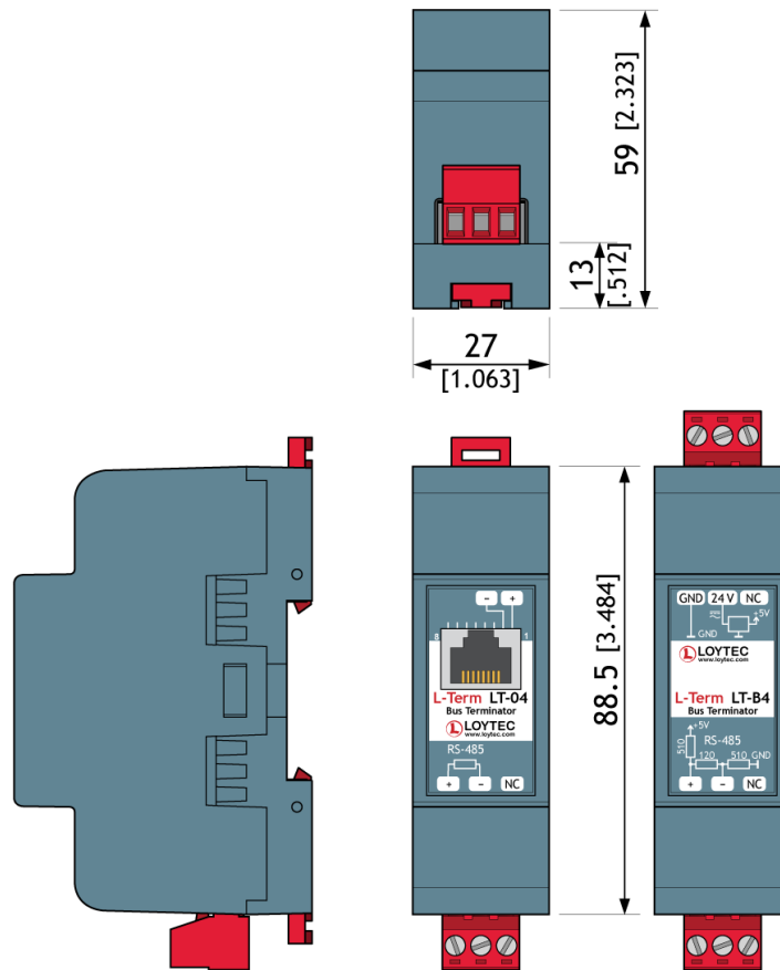
Figure 141: RS-485 Network Termination.
