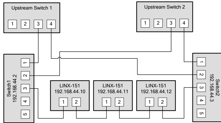
Figure 144: Ring Ethernet topology
