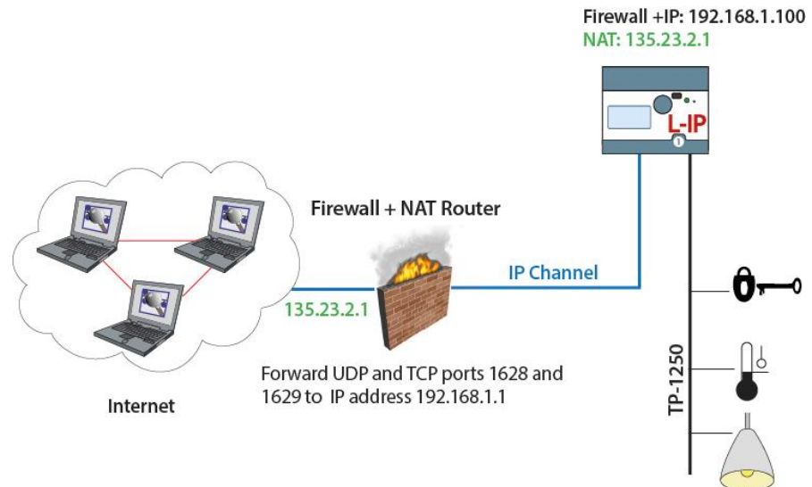
Figure 85: Operating an L-IP behind a NAT router and firewall.
