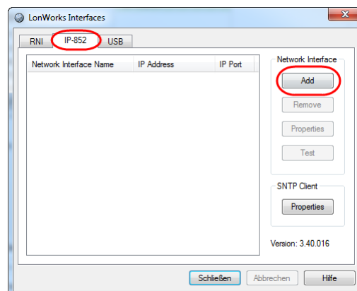
Figure 91: Add a new LNS IP interface to your PC.
