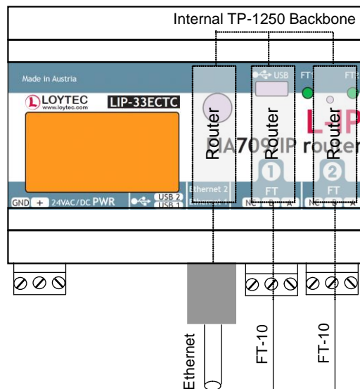
Figure 89: Internal structure of the multi-port L-IP in configured CEA-709 router mode.
