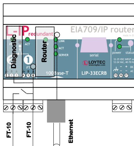
Figure 100: Internal structure of the L-IP Redundant
