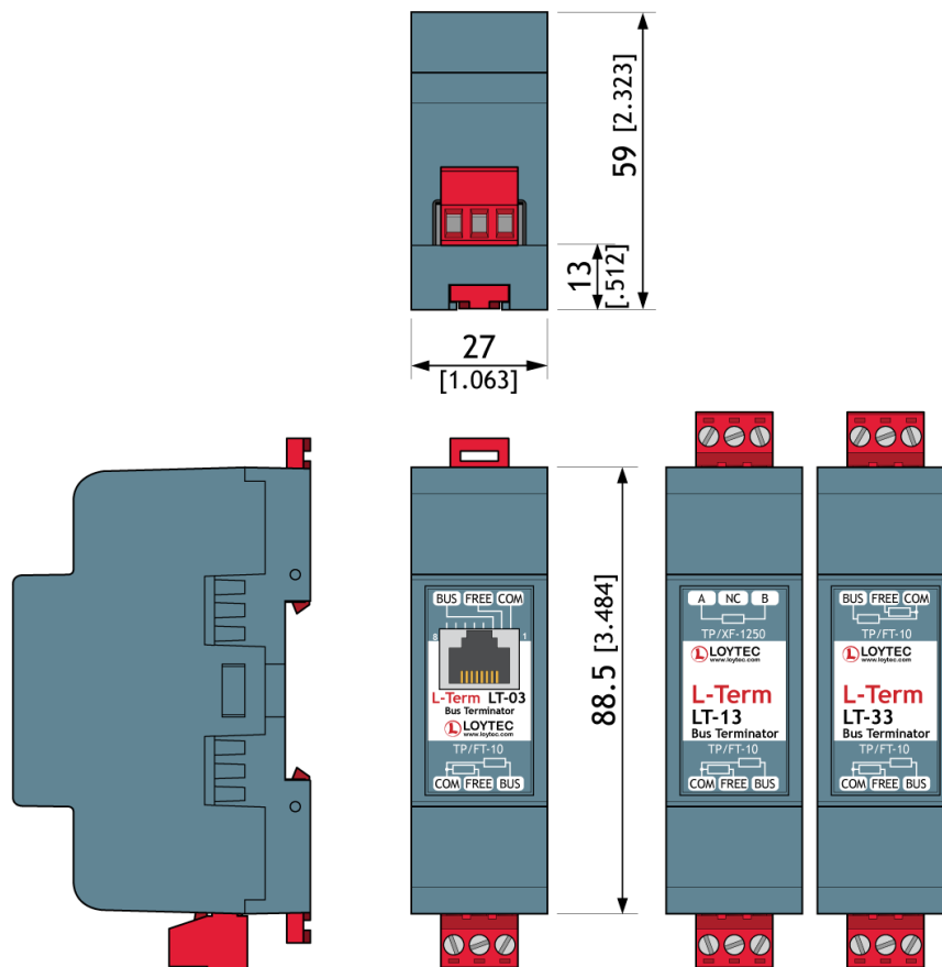
Figure 140: FT-10 Network Termination.
