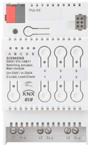
N 513/11 SWITCH ACTUATOR MAIN MODULE 3X AC 230V, 20AX C-LOAD, LOAD CURRENT MONITORING
