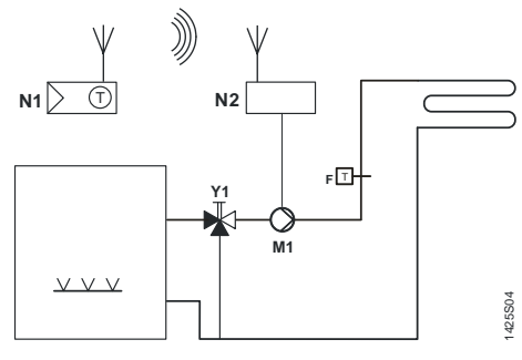
Room thermostat with direct control of hydronic floor heating system
