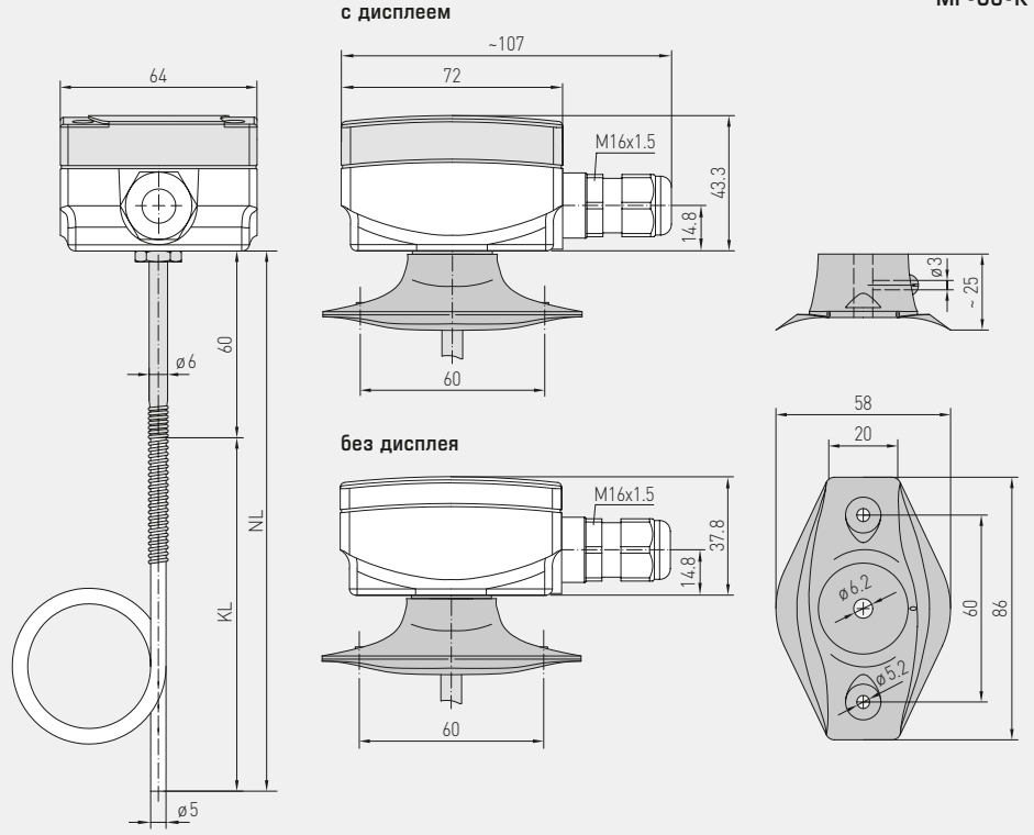
MWTM-Modbus MF-06-K
